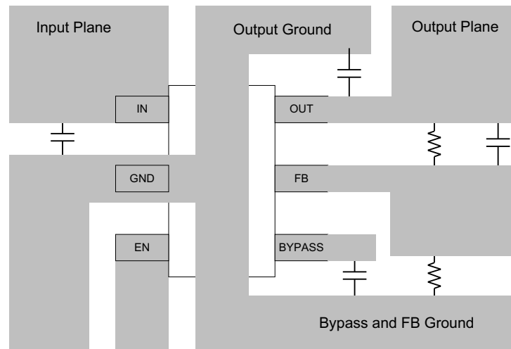
Figure 7-7. Layout Example (DBV 6-Pin Package)
