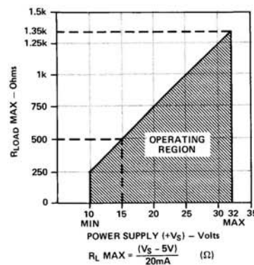
Figure 1. Maximum Load Resistance vs. Power Supply
