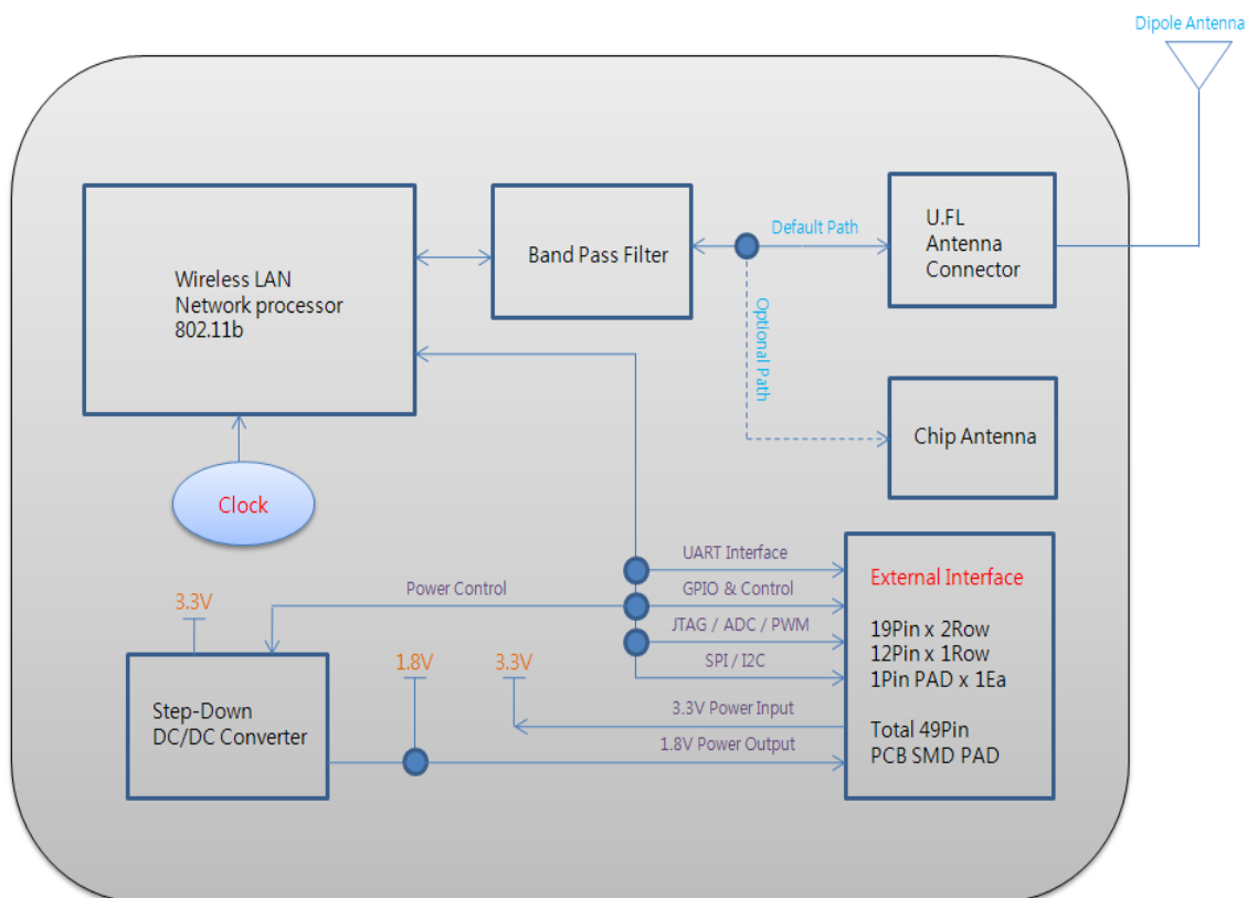
Figure 2. Block Diagram
