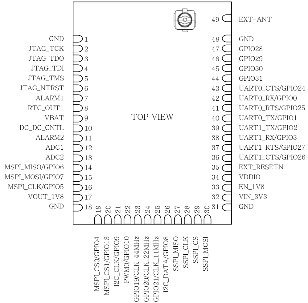
Figure 3. Pin description
