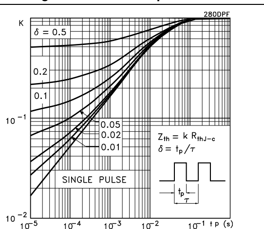
Figure 3. Thermal impedance
