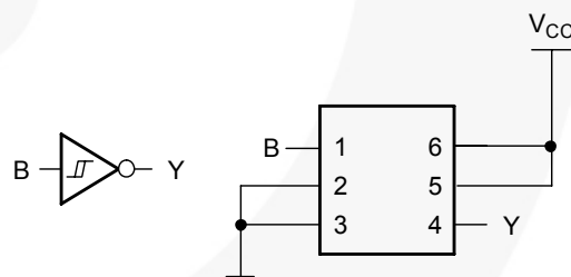
Figure 7. Inverter
