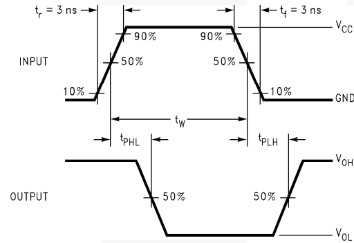
Figure 10. AC Waveforms
