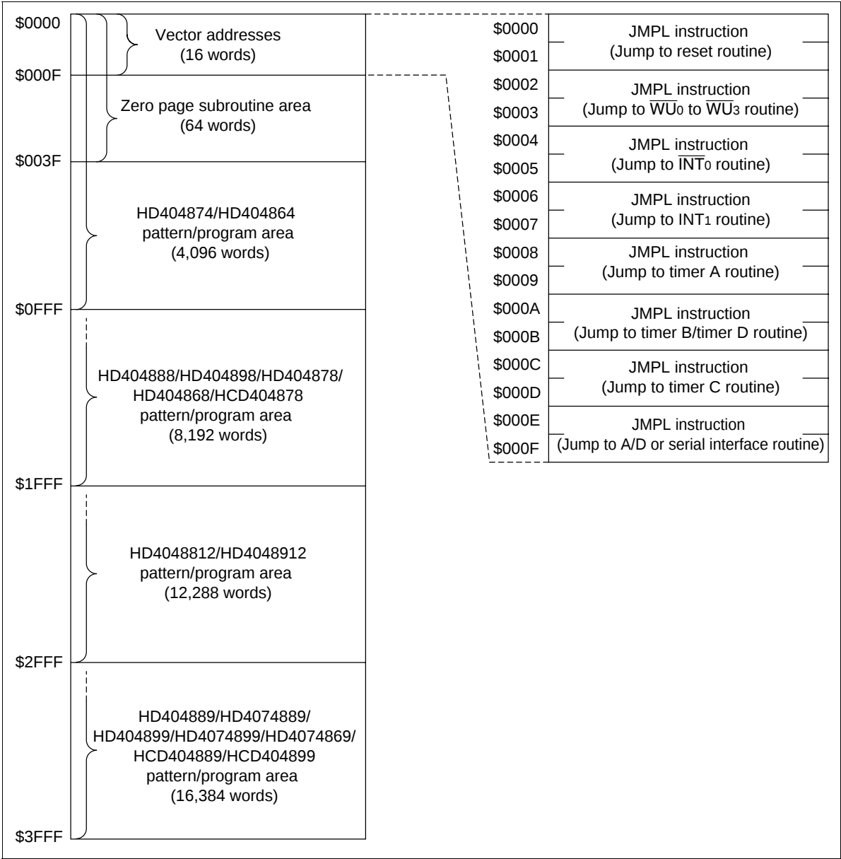
Figure 1 ROM Memory Map
