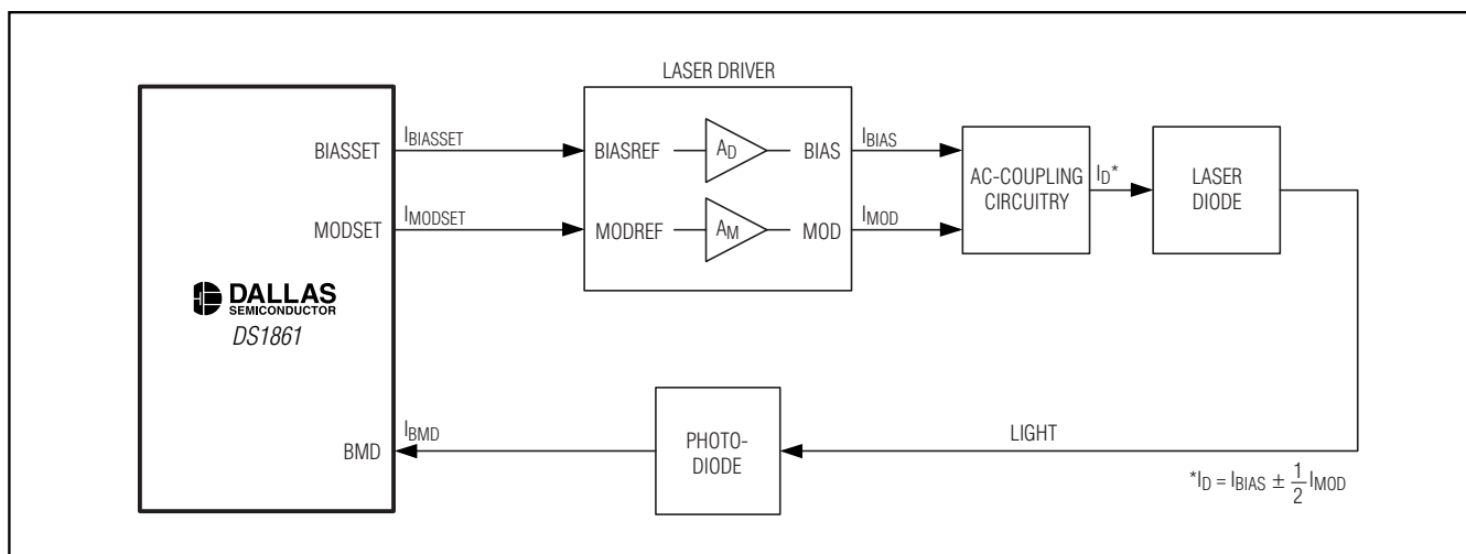
Figure 8. AERC Block Diagram
