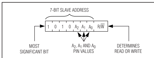
Figure 15. Slave Address Byte
