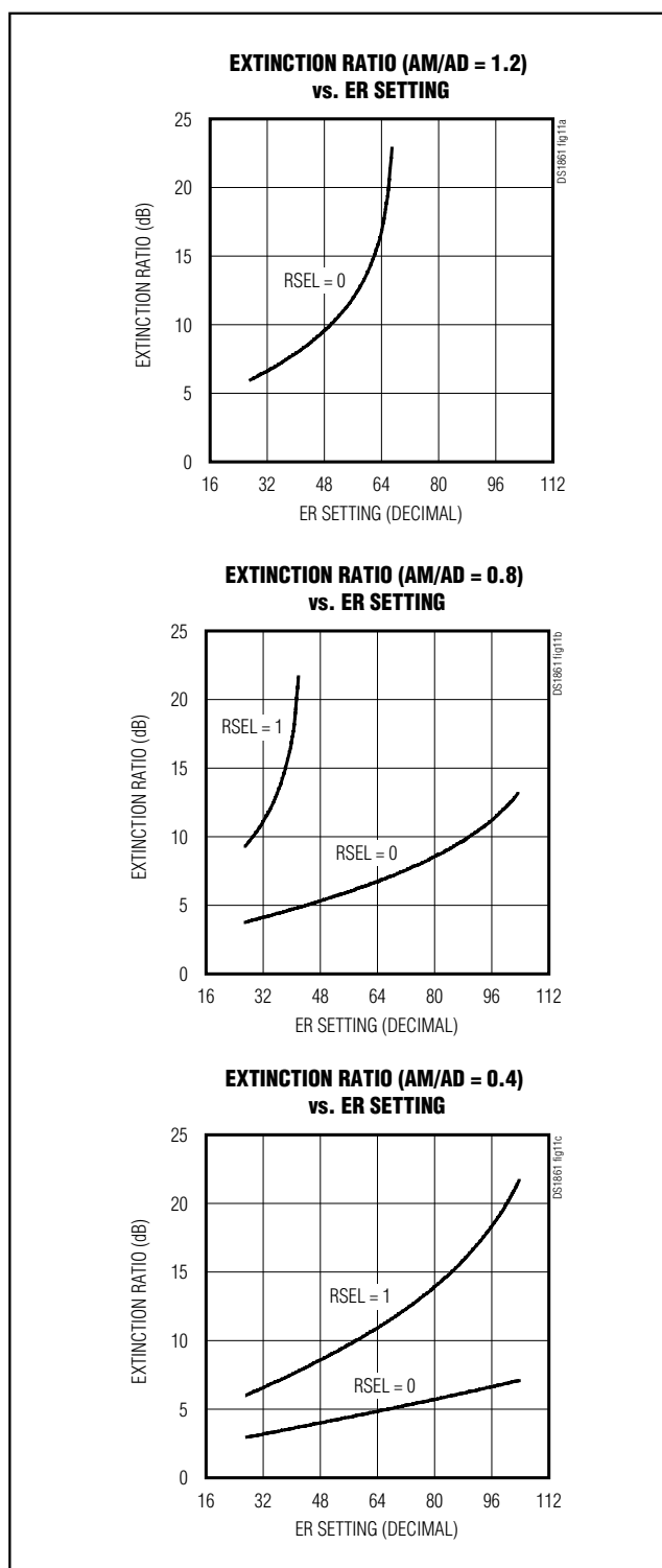
Figure 11. Typical Extinction Ratios vs. N Codes
