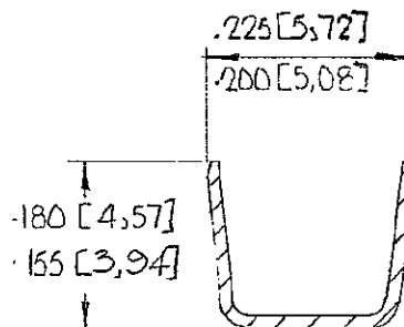
SECT. BB
