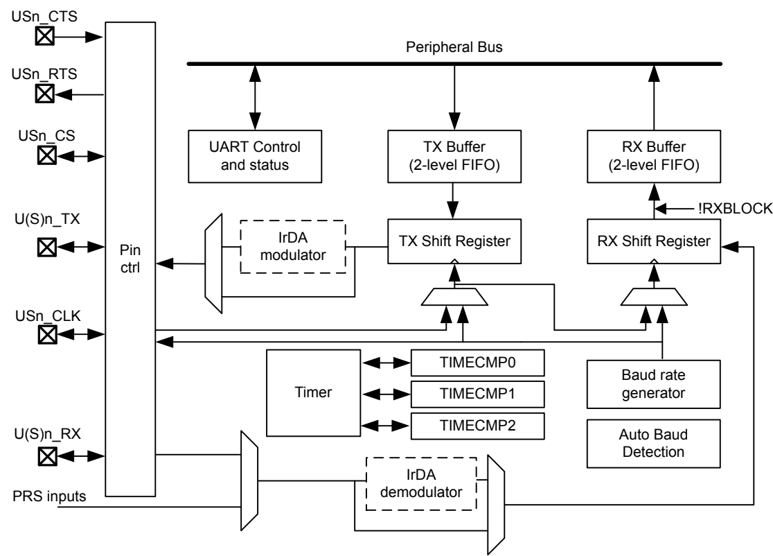
Figure 18.1. USART Overview
