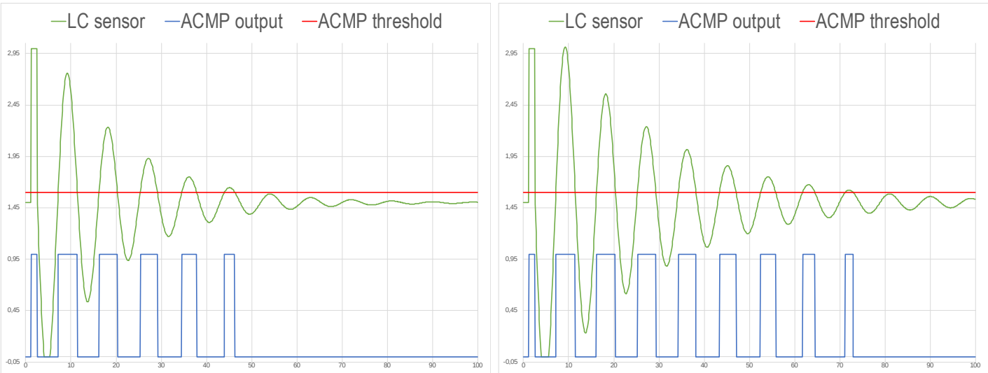
Figure 28.17. LC Sensor Oscillations
