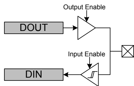
Figure 32.3. Push-Pull Configuration
