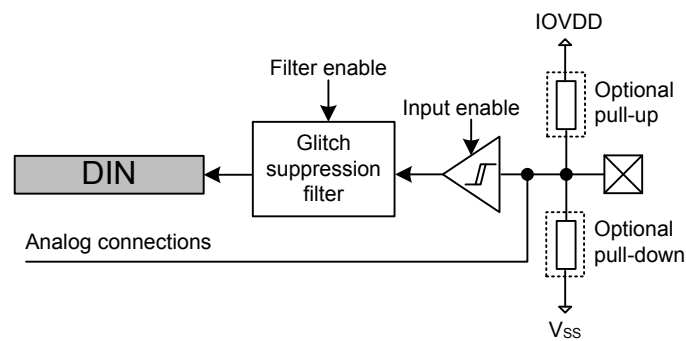
Figure 32.2. Tristated Output With Optional Pull-up or Pull-down
