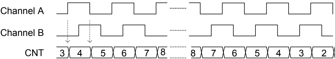
Figure 20.8. TIMER/WTIMER X2 Decoding Mode
