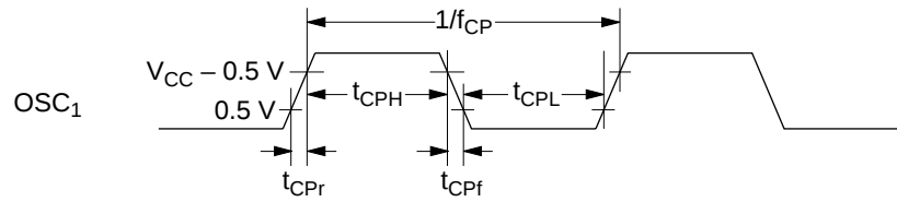
Figure 43 Oscillator Timing
