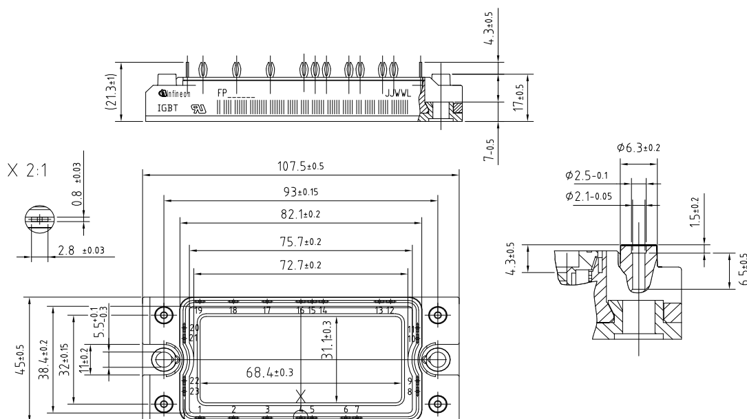
PCB hole pattern
