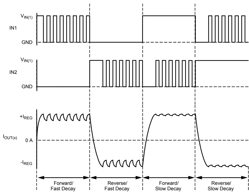
PWM Control Timing Diagram
