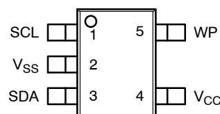
TSOT-23 (TD), TSOP-5** (TS) (Top View)
