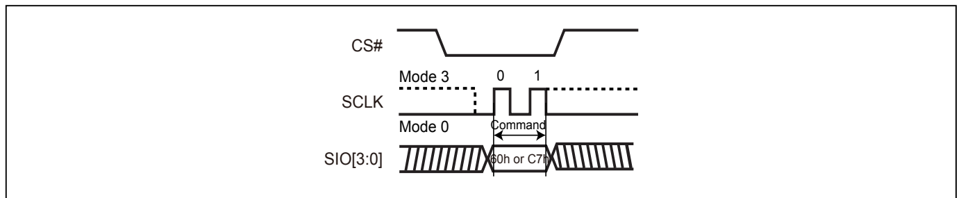
Figure 43. Chip Erase (CE) Sequence (QPI Mode)
