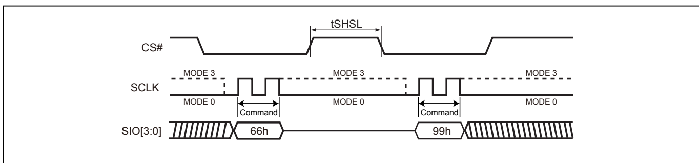
Figure 57. Reset Sequence (QPI mode)
