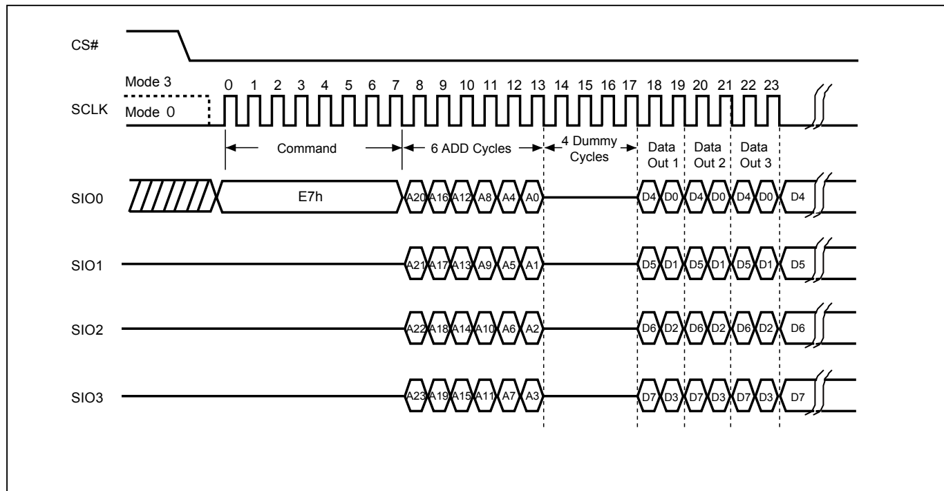
Figure 31. W4READ (Quad Read with 4 dummy cycles) Sequence
