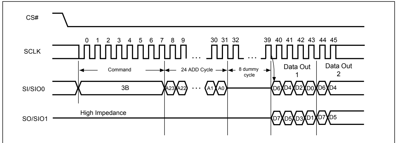
Figure 26. Dual Read Mode Sequence (Command 3B)
