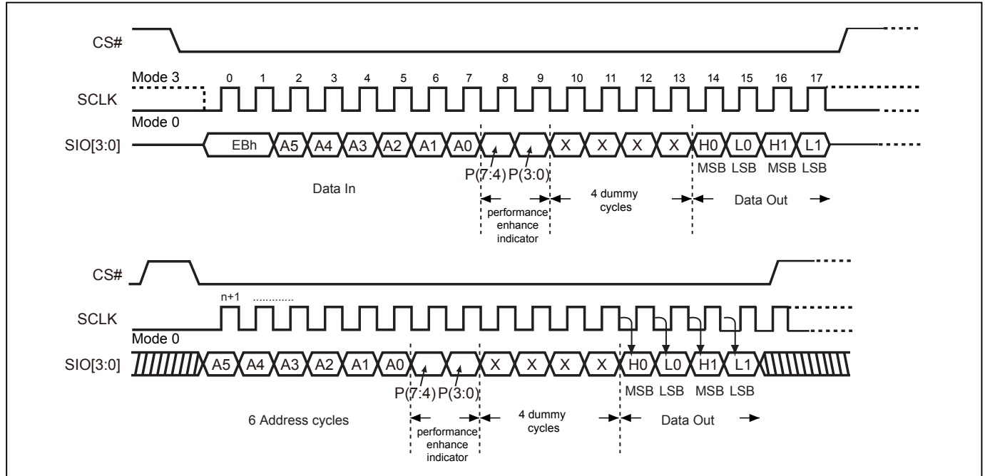
Figure 35. 4 x I/O Read Performance Enhance Mode Sequence (QPI Mode)
