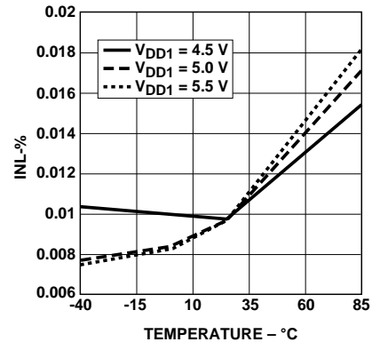
Figure 4. INL (%) vs. Temperature.
