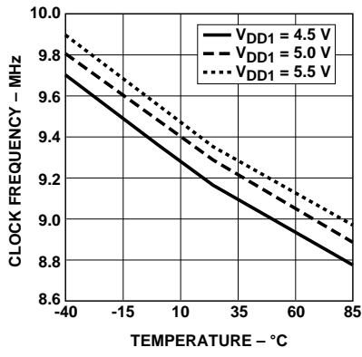
Figure 17. Clock Frequency vs. Temperature.
