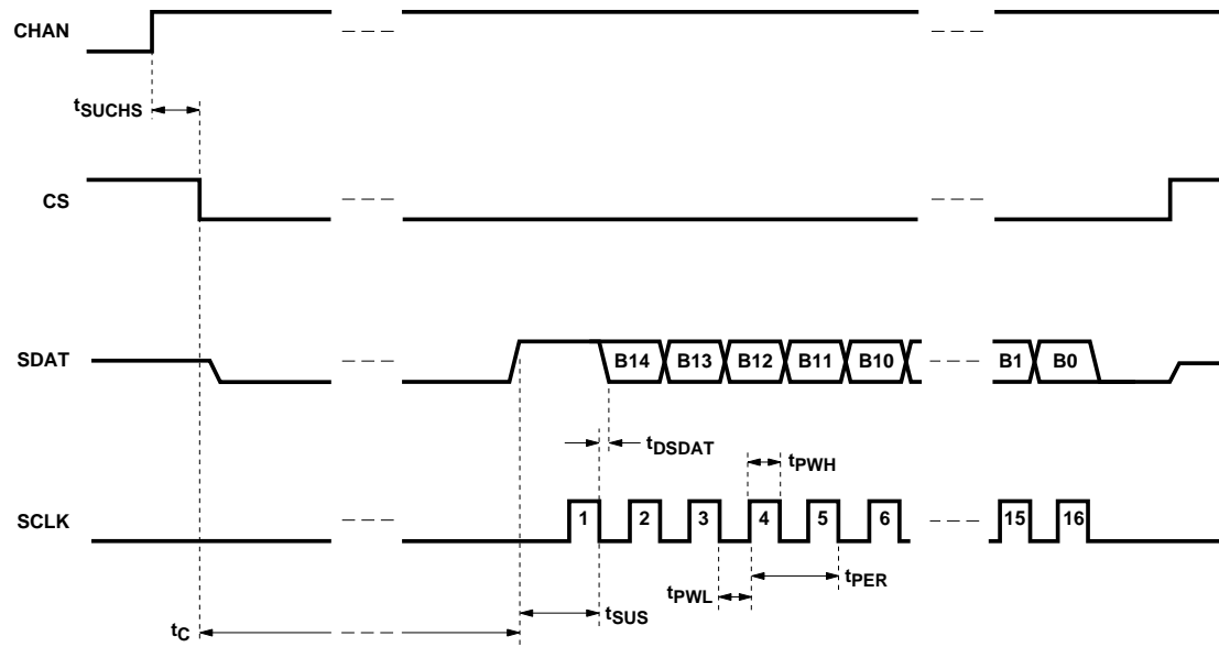
Figure 19. Conversion Timing.
