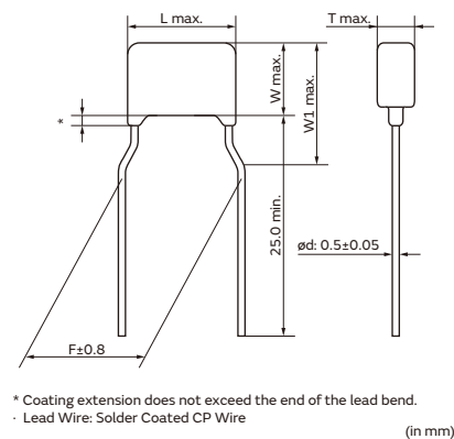
Dimensions code: 2/3/4 Lead style code: K1
