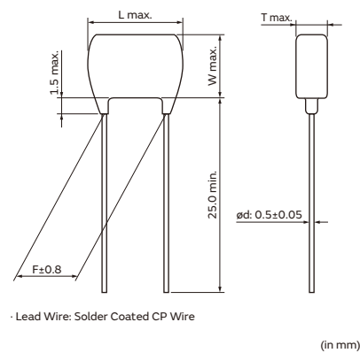
Dimension code: 2 Lead style code: A2
