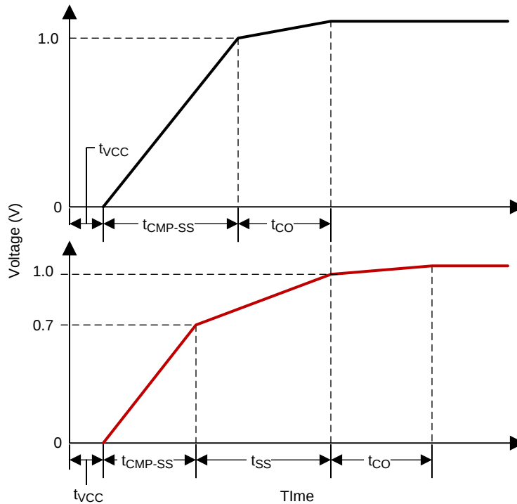
Figure 14. Start-up Waveforms
