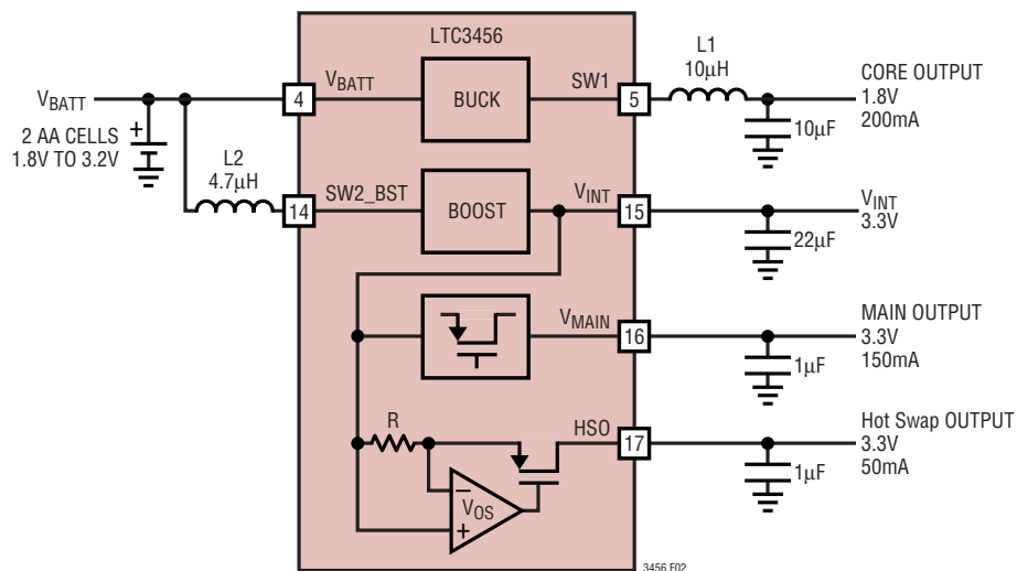
Figure 2. Battery-Powered LTC3456
