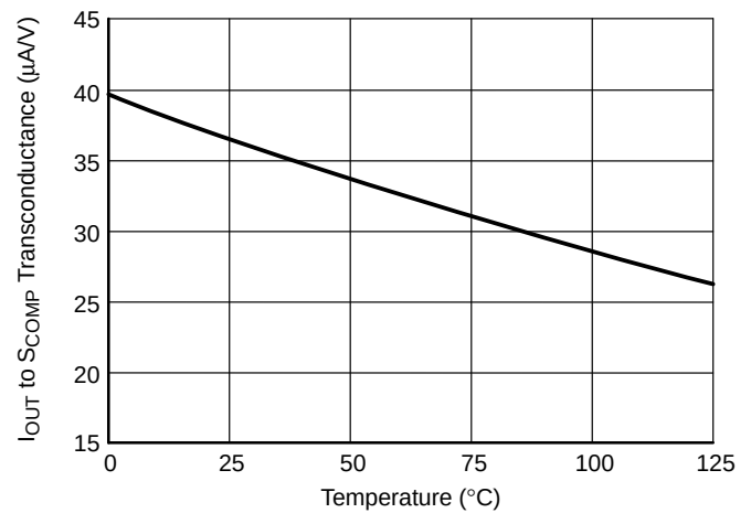
Figure 23. IOUT to SCOMP Transconductance vs. Temperature
