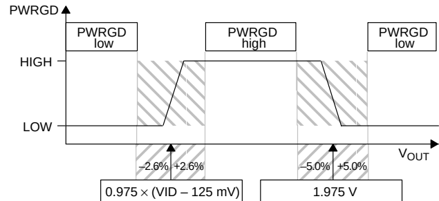
Figure 33. PWRGD Assertion Window
