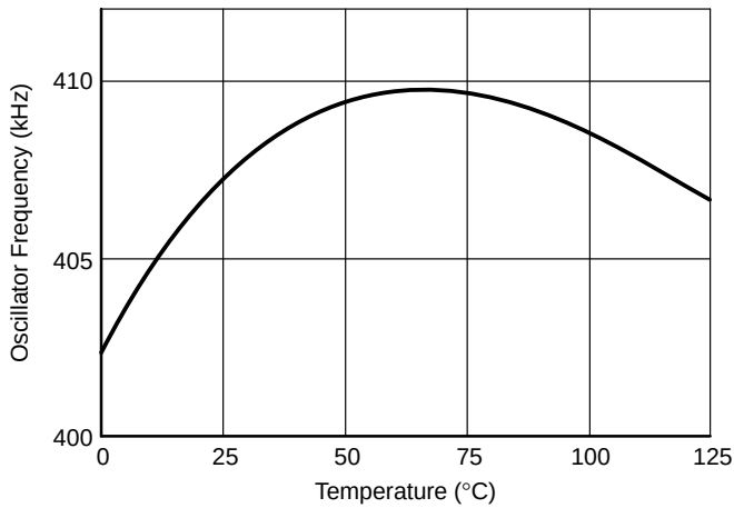
Figure 8. Oscillator Frequency vs. Temperature for R_{OSC} = 32.4 k \Omega
