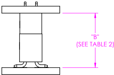
FIG 2 IPT1-01-D-VS MATED WITH IPS1-X1-D
