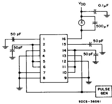
Fig. 13—Dynamic power dissipation test circuit.
