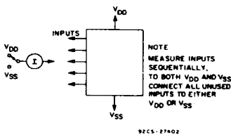
Fig. 7 - Input current test circuit.
