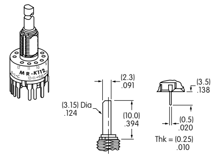
Shaft Terminal
