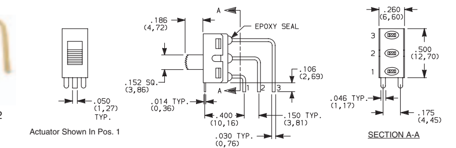
1101M2S3AV2BE2 Vertical Actuation SPDT
