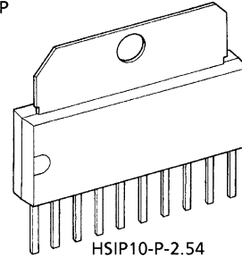
TA7291S/SG
