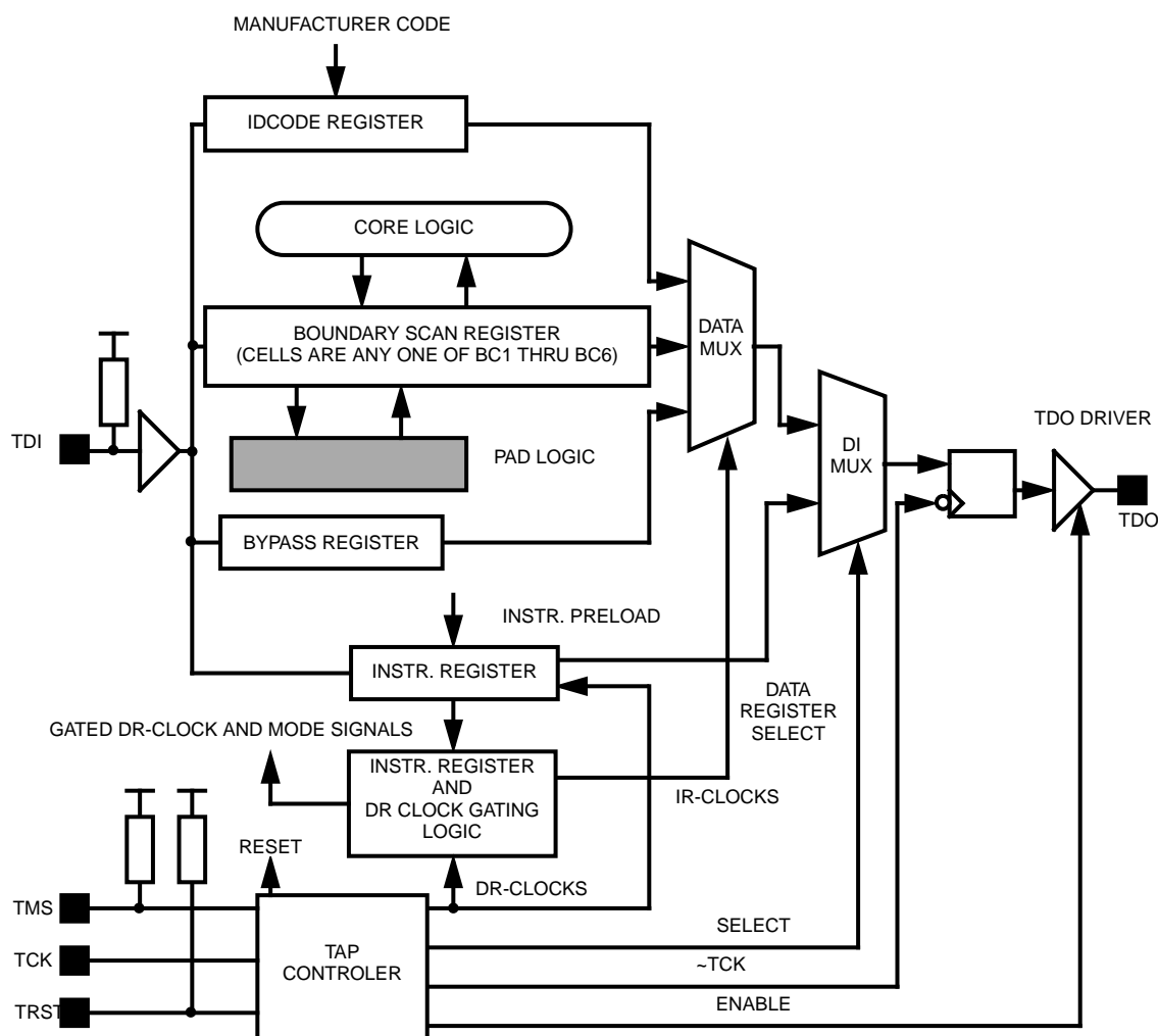
FIGURE 18. TIEEE 1149.1 Architecture
