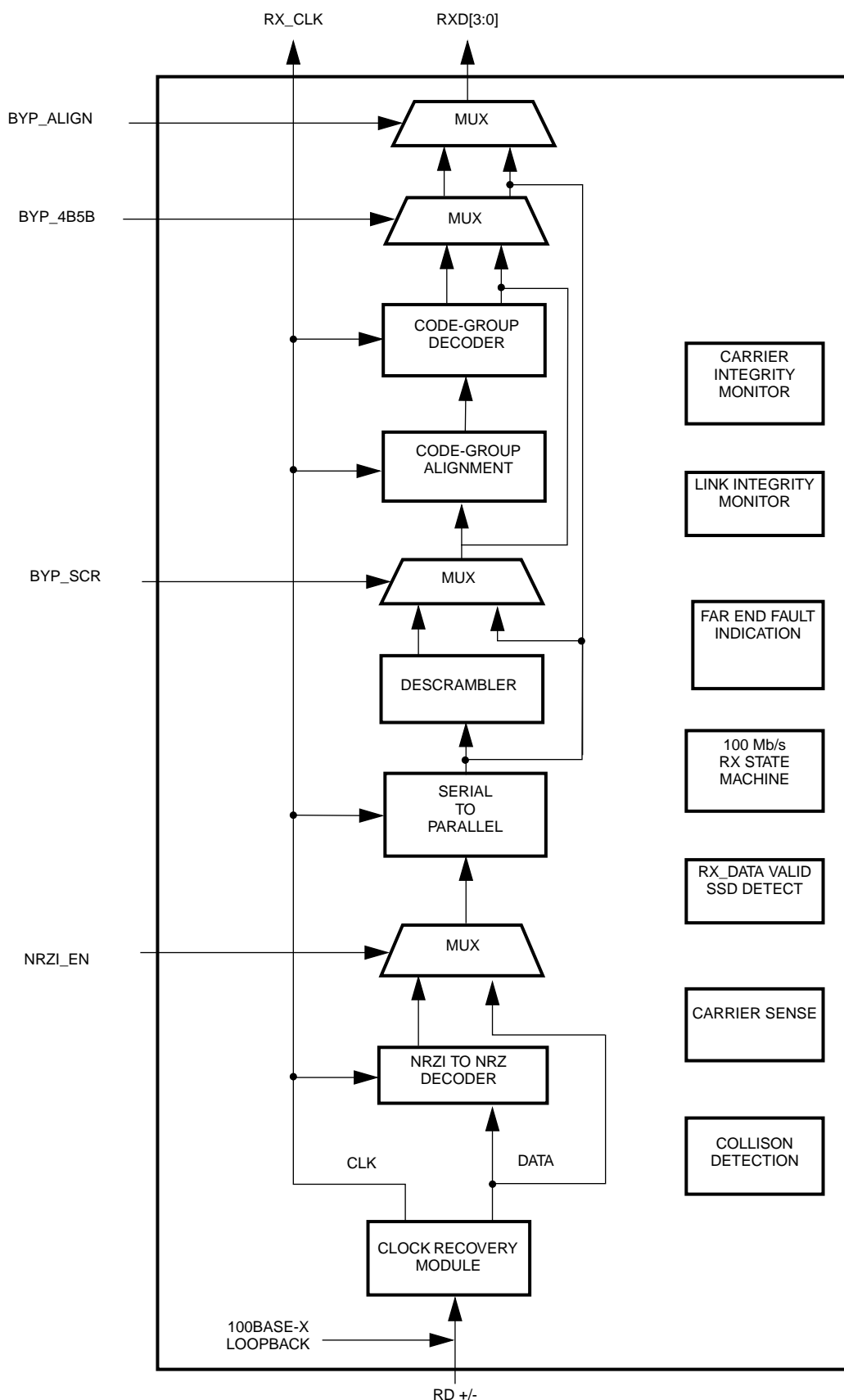
FIGURE 5. 100BASE-X Receiver
