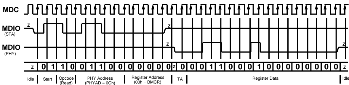
FIGURE 2. Typical MDC/MDIO Read Operation
