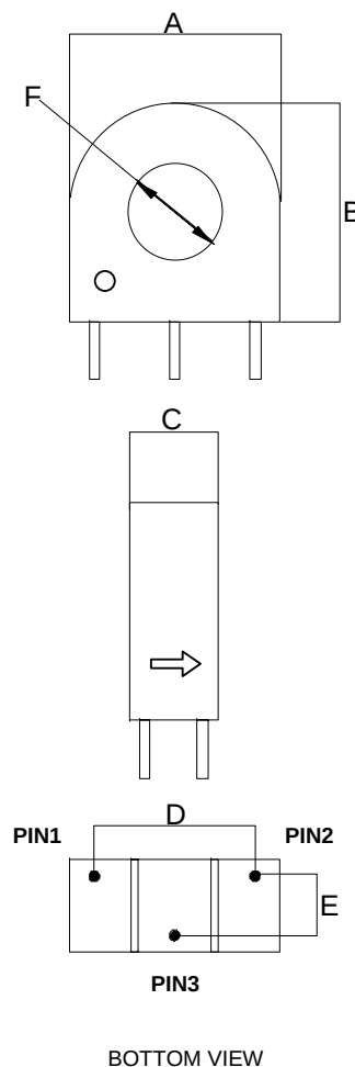
BOTTOM VIEW
