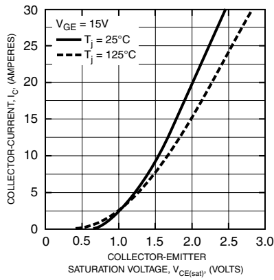
COLLECTOR-EMITTER SATURATION VOLTAGE CHARACTERISTICS (BRAKE PART - TYPICAL)
