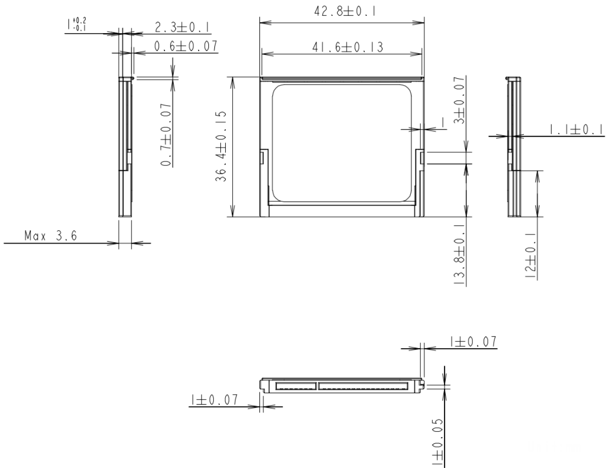
FIGURE 8-1: Physical dimension
