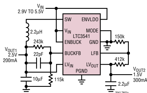
LTC3541 Typical Application
