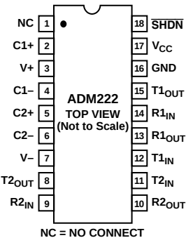
Figure 8. ADM222 DIP and SOIC Pin Configurations
