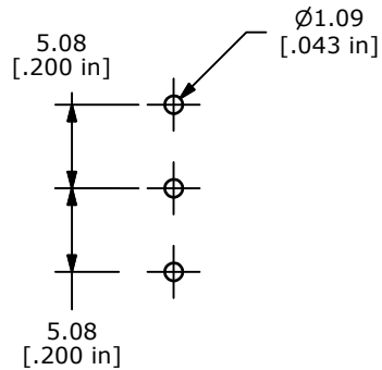
P.C. MOUNTING
