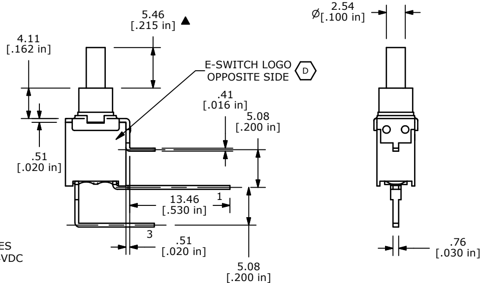
CIRCUIT: SPST
