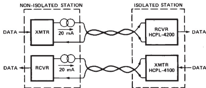
Figure 21. Full Duplex Point-to-Point Current Loop System Configuration.
