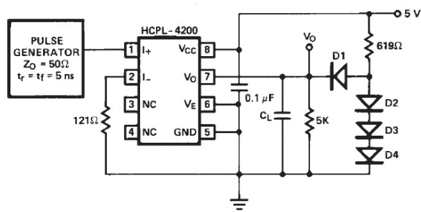
V_{IN} = 5 \text{ VOLT} , 100 KHz 10% DUTY CYCLE D1 - D4 ARE 1N916 OR 1N3064 C_L = 15 \text{ pF} INCLUDING PROBE AND JIG CAPACITANCE
