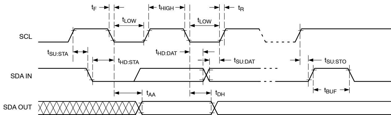
Figure 5. Bus Timing
