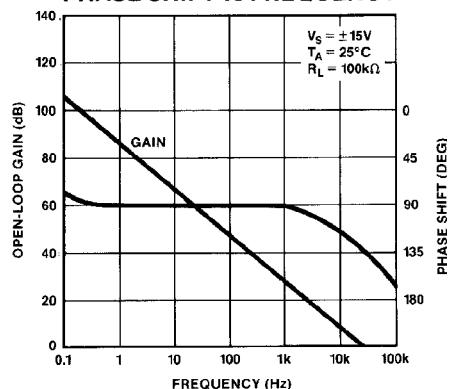
OPEN-LOOP GAIN AND PHASE SHIFT vs FREQUENCY
