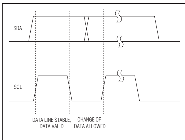
Figure 5. Bit Transfer
