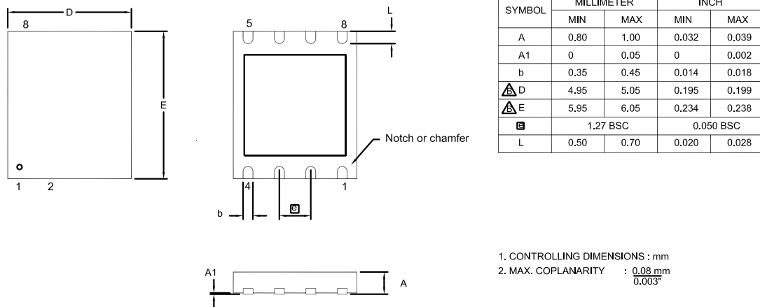
Figure 41. 8-Pin Quad Flat No-Lead Package (QFN)/MLF-S
