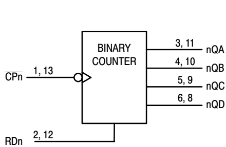
Figure 2. Logic Diagram
