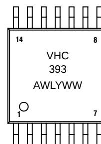
TSSOP-14 DT SUFFIX CASE 948G
