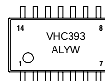
SOIC EIAJ-14 M SUFFIX CASE 965
