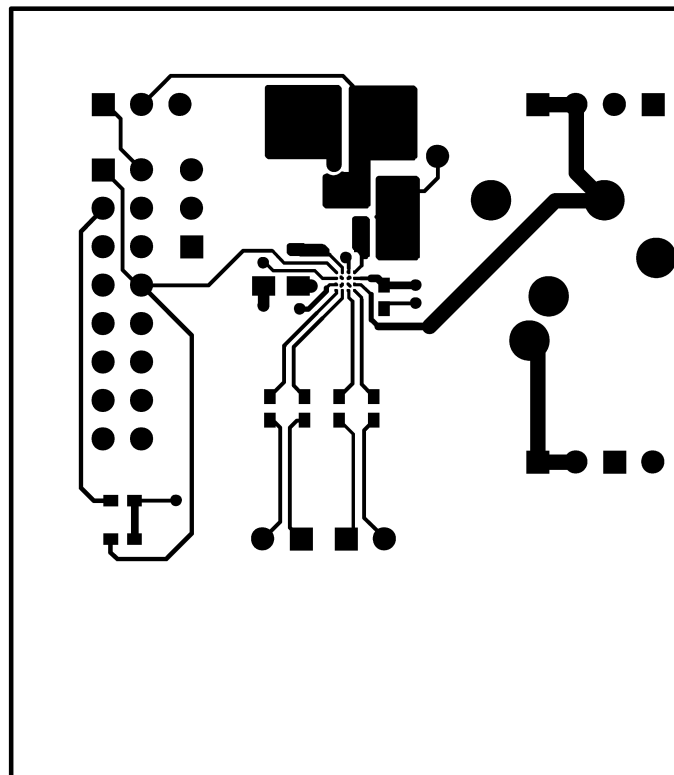
Figure 39. Top Layer
