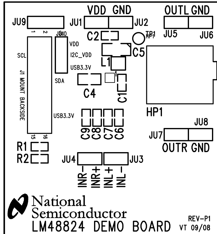
Figure 38. Top Silkscreen
