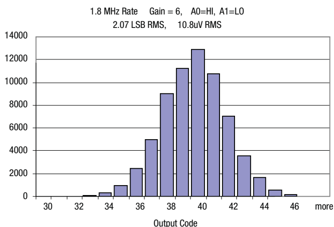
ADCDS-1603 Grounded Input Histogram – 1.8 MHz Rate
