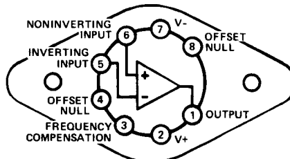
TO-3 STYLE BOTTOM VIEW
