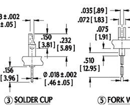
③ SOLDER CUP
