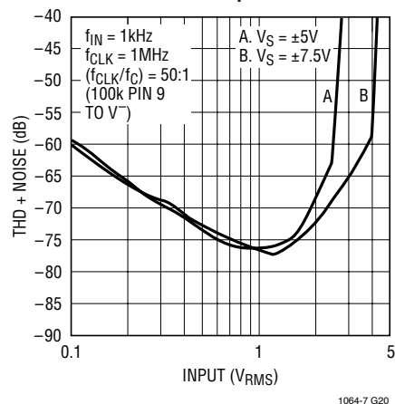
THD + Noise vs Input
