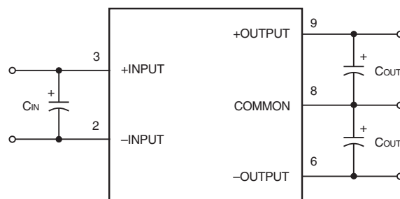
Figure 7. Using External Capacitors to Reduce Input/Output Ripple/Noise
