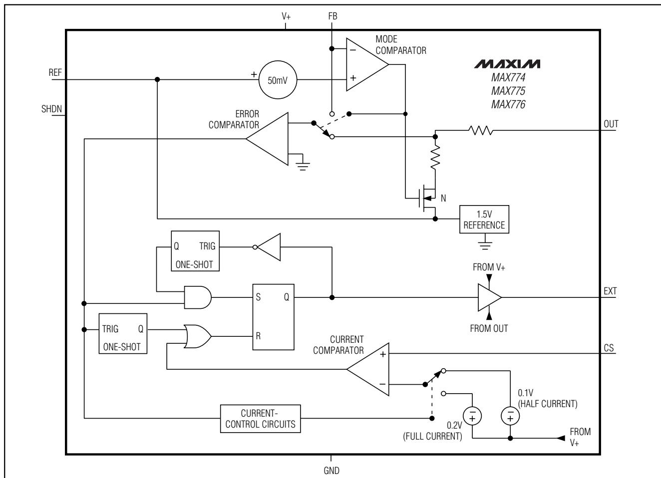
Figure 1. Functional Diagram
