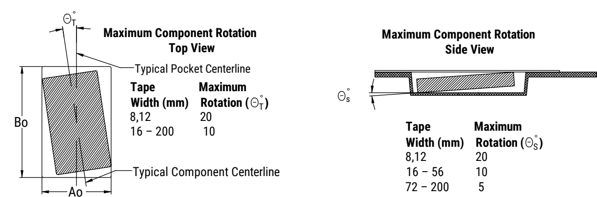
Figure 3 – Maximum Component Rotation
