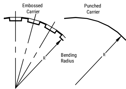
Figure 5 – Bending Radius
