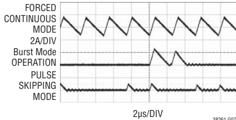
FIGURE 13 CIRCUIT V OUT = 3.3V I LOAD = 100µA
