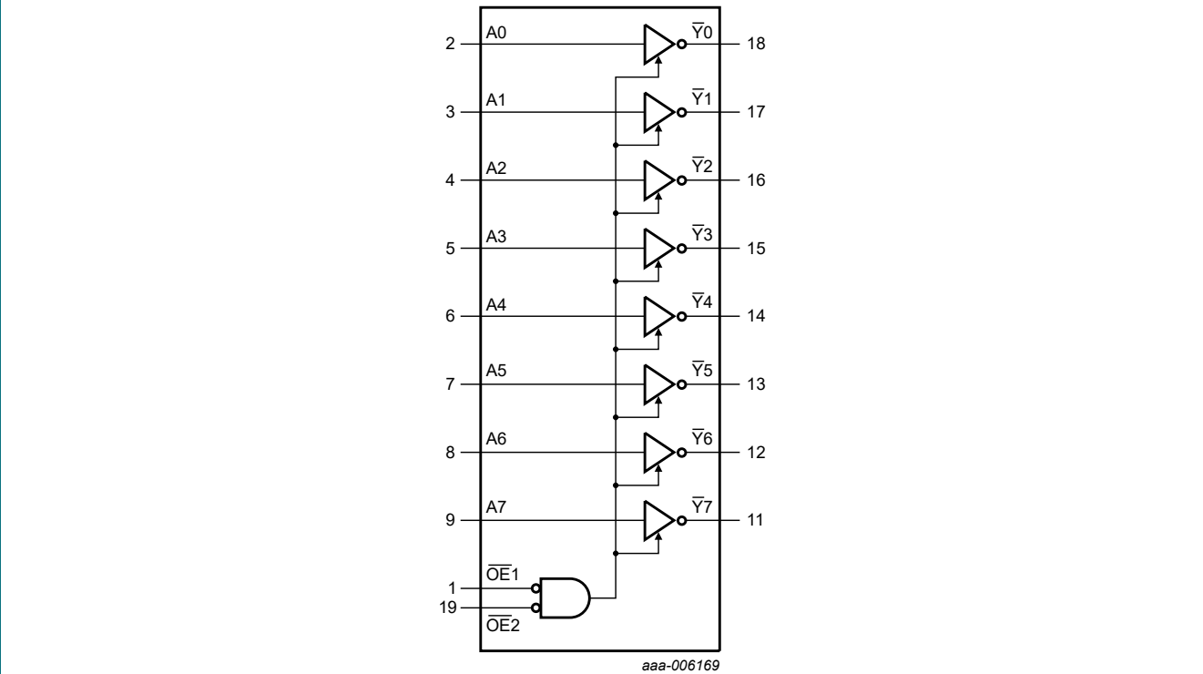
Fig. 3. Functional diagram
