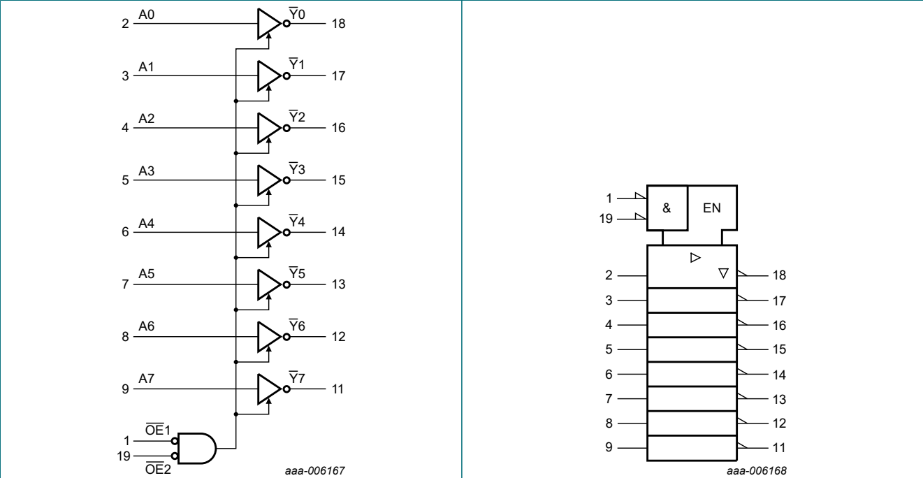
Fig. 1. Logic symbol
