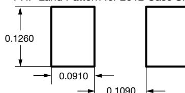
PHP Land Pattern for 2512 Case Size
