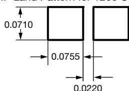
PHP Land Pattern for 1206 Case Size
