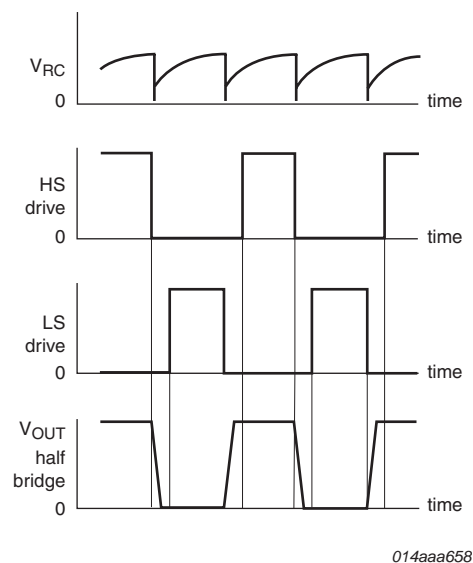
Fig 4. Oscillator, drivers and output signals
