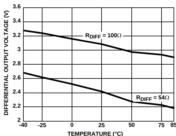
FIGURE 7. DRIVER DIFFERENTIAL OUTPUT VOLTAGE vs TEMPERATURE
